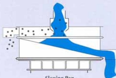
Sloping Pan
