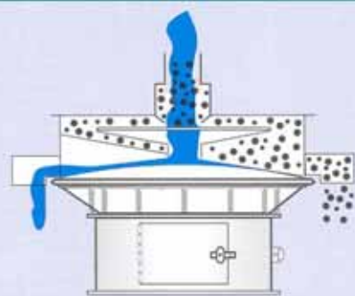
Auxiliary-Series
